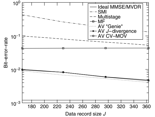
Figure 13. BER versus data record size (the signal model is the same as in Fig. 12, and \text{SNR}_0 = 8 dB).
