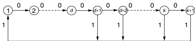
Figure 9. FSTD for RLL( d, k )-constrained sequences.
