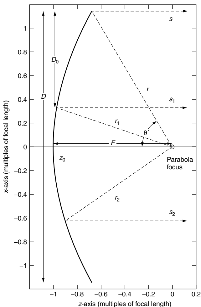
Figure 3. Parabolic single-reflector geometry, with offset section shown.
