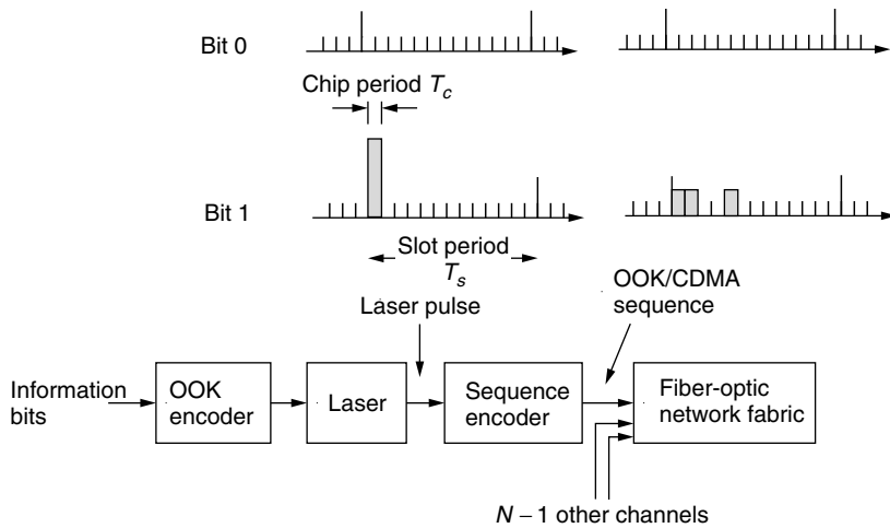
Figure 1. The transmitter block diagram of a direct-detection optical OOK CDMA system.
