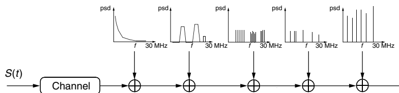
Figure 7. Noise types present in the PLC environment.
