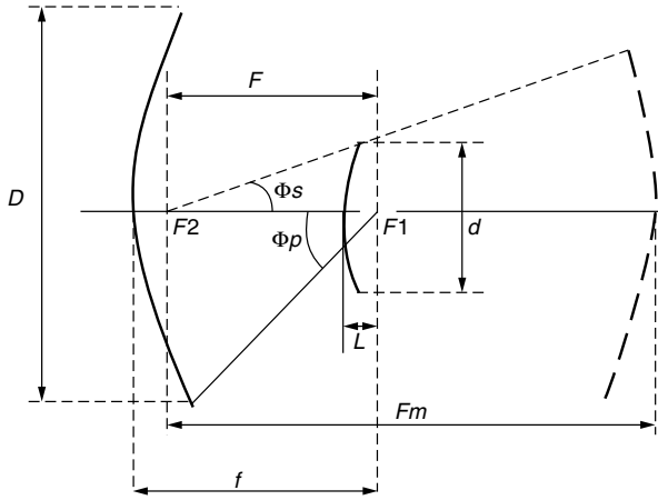
Figure 4. Antenna parameters.
