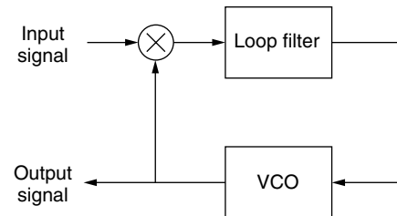
Figure 10. Phase-locked loop.
