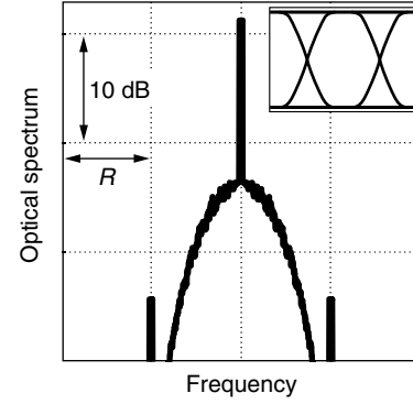
Figure 3. Optical spectrum and eye diagram of an NRZ signal.
