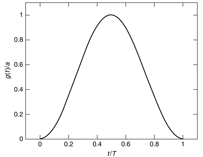
Figure 6. Raised-cosine pulse.
