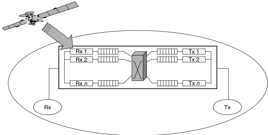
Figure 2. An example of satellite with onboard processing and switching facilities.
