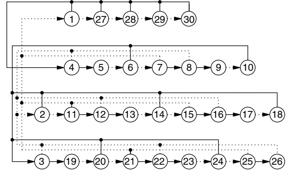
Figure 12. FSTD for MTR(j=2, k=7, t=4) constrained sequences. Solid line: 1, dotted line: 0.
