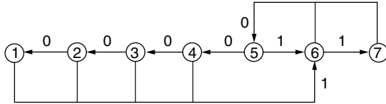
Figure 11. FSTD for MTR(j=2, k=5) constrained sequences.
