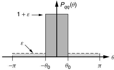
Figure 17. Power spectrum of band-limited white noise with \varepsilon white-noise overlay.
