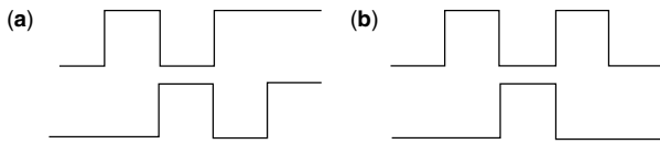
Figure 13. Error patterns eliminated by the j = 2 constraint. (a) Tribit shift, (b) quadbit to dibit.
