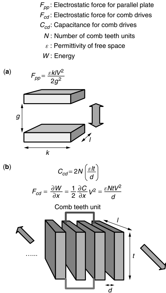
Figure 11. Electrostatic designs: (a) parallel-plate capacitor, (b) comb drives.
