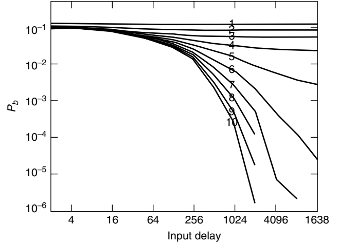
Figure 12. Simulated performance of the SCCC employing a nonrecursive outer encoder described in Section 5.2.2. The bit error probability is plotted versus input decoding delay for different number of iterations. The signal-to-noise ratio is 0.75 dB.
